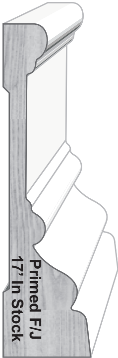
RWCA-23R/DELTA 15/16" X 3-1/2"
