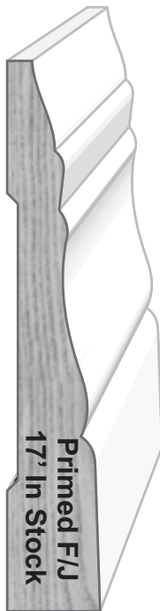
RWCA-69/366 11/16" X 3-1/4" Primed F/J 17' In Stock
