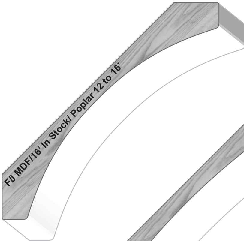
R=3-3/4" P=3-3/4" 45°
