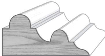
RWPA-62 3/4" X 1-9/16"
