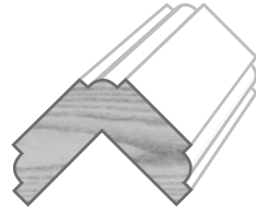
RWCN-02 3/4" OS 5/8" X 7/8" RUN SIZE
