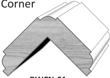
RWCN-01 1 3/8" OS 1-1/16" X 1-5/8" RUN SIZE
