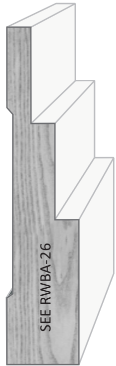
RWCA-44 3/4" X 3-1/2"
