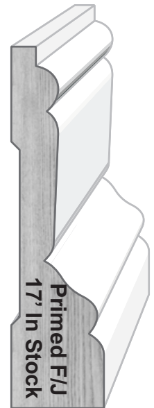
RWCA-72 / WM462 11/16" X 2-3/4" Primed F/J 17' In Stock
