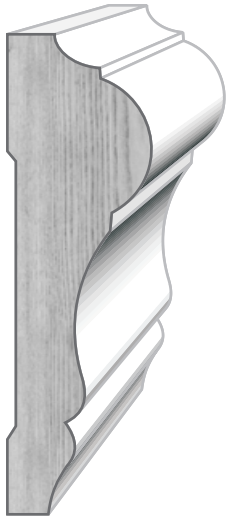
RWCH-02 3/4" X 2-1/2"
